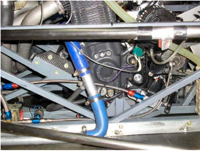
General view of air line from LP regulator to actuator
